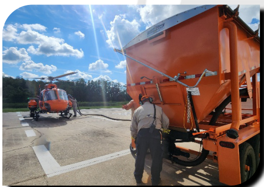
Picture 7: Autoloader dispensing treatment material
